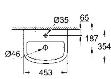
39 424 000 Handrinse basin 45 cm
