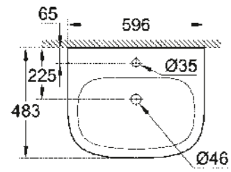
39 337 000 39 337 00H* Countertop basin 60 cm
