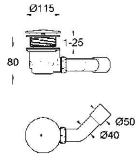
49 534 000* Waste set horizontal for Universal shower trays
