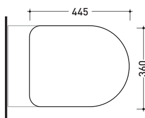
art. AP118 - AP118G vista zenitale / zenital view
