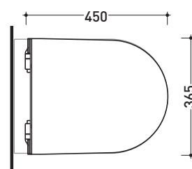
art. AP119 - AP119G vista zenitale / zenital view
