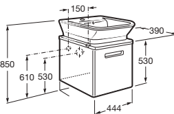
Base unit to suit 350 basin.
