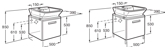
Base unit to suit 500 basin.
