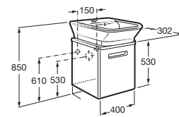
Base unit to suit 400 basin.
